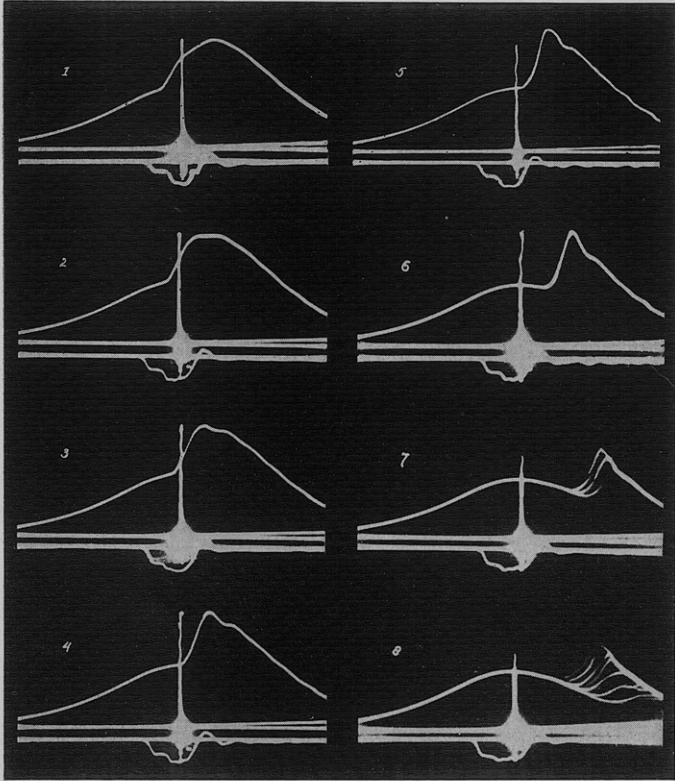
FIG. 22. Series of diagrams with increasing delays (1 to 8)
