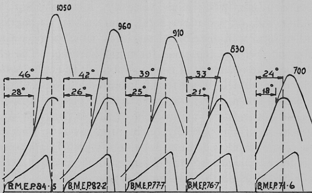
FIG. 23. Smooth pressure rise notwithstanding long delays
